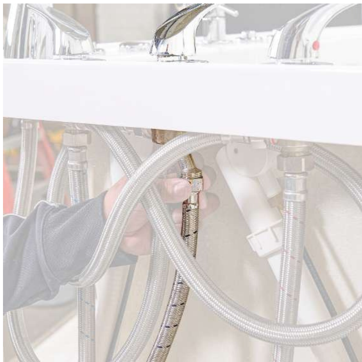
Tighten the other end of the supply hose on the available spot underneath the center valve (diverter) of the 5pc faucet
